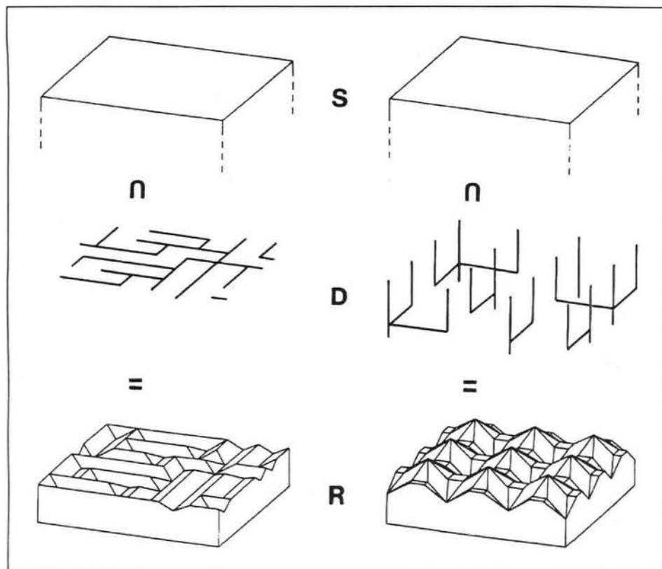
Figure 1. The Pure Karst Model presented in the terms of set theory. Fluvial relief is shown on the left side, karst relief on the right. S = initial surface; D = drainage system; R = the intersection of S and D . The symbol " \cap " is the mathematical symbol for "intersection".
